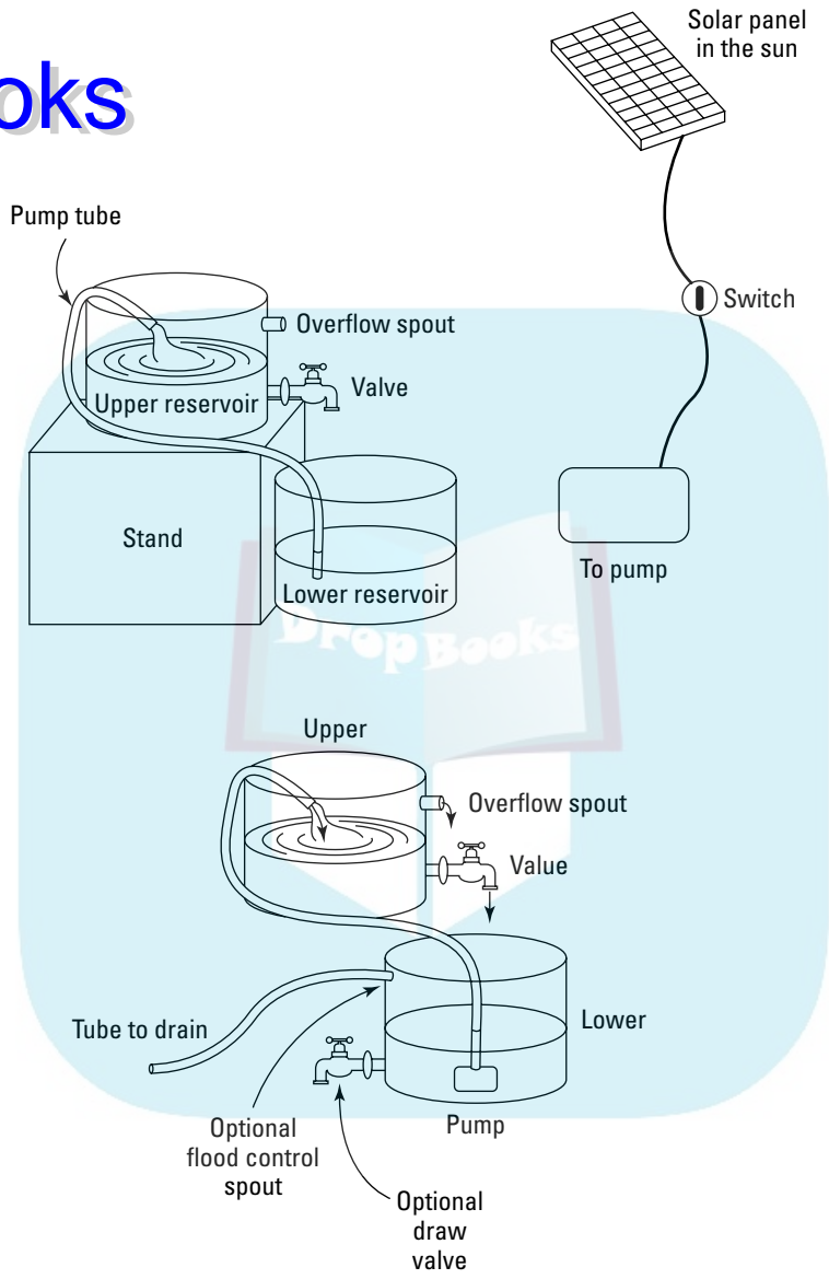
Figure 8-1: A wooden barrel solar fountain.
